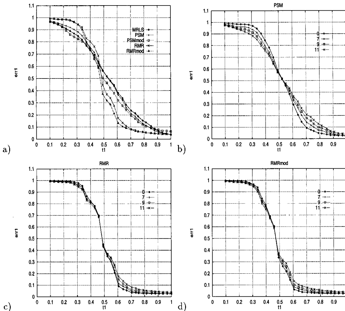
FIG. 10. (a) Average error \overline{err}_1 obtained for each of the five algorithms as a function of the percentage t_1 of the support window W occupied by area Z_1 , with a zero-mean Gaussian white noise of standard deviation \sigma_G = 11 added to the constructed images. (b)–(d) Average error \overline{err}_1 as a function of t_1 for different values of the standard deviation \sigma_G of the Gaussian noise, for, respectively, the algorithm (b) PSM, (c) RMR, and (d) RMRmod.
